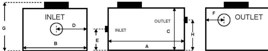
MODEL CN6T ~ 6 Million Btuh
